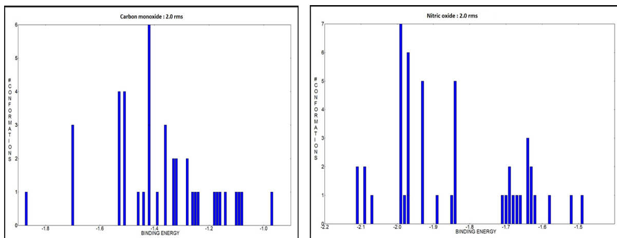
Figure S4-. Histogram showing multiple Conformations of Carbon monoxide and Nitric oxide
