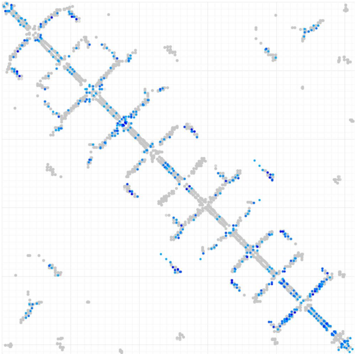
Figure S1-Gremlin 1V54 contact map in 2D representation of 3D protein structure (Grey filled circles underneath were PDB residue contacts, Blue filled circles are Gremlin results)
